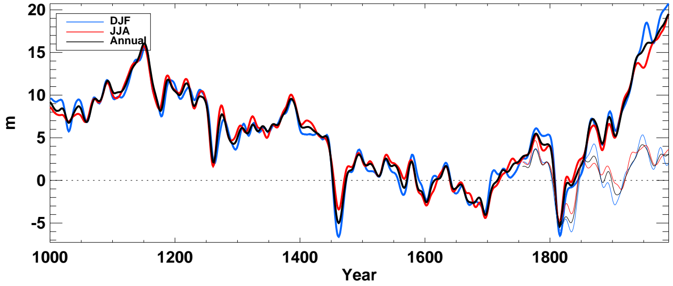
z500_ from echo-g averaged over SH ocean
