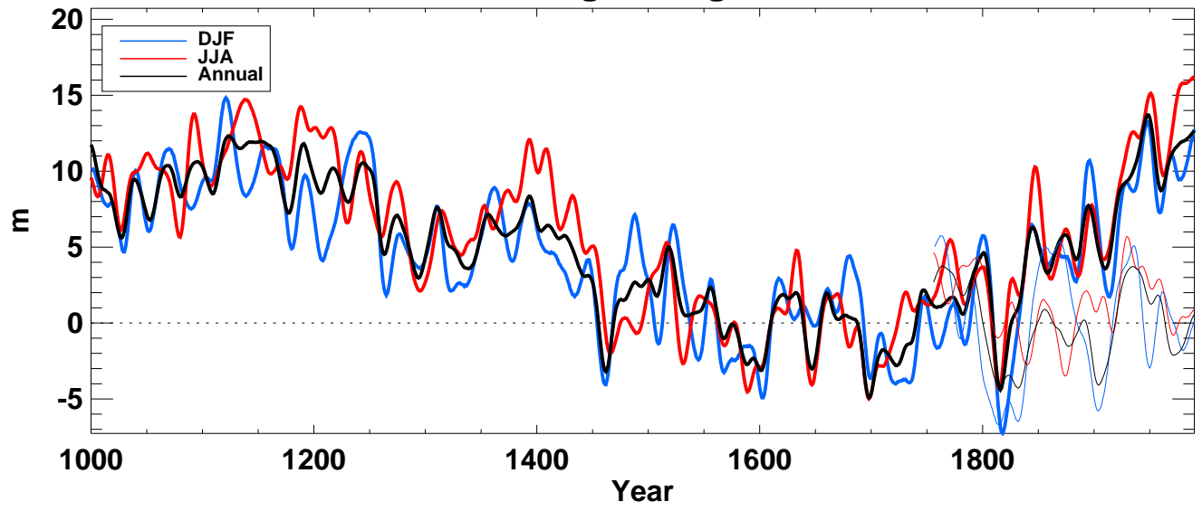
z500_ from echo-g averaged over SH land
