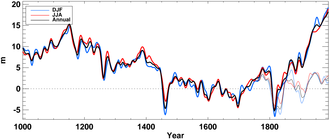
z500_ from echo-g averaged over SH full
