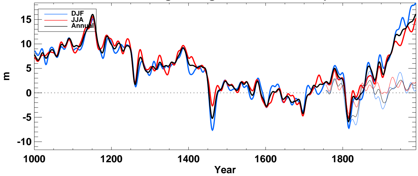
z500_ from echo-g averaged over S-extratropics ocean
