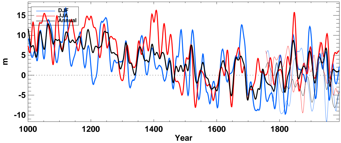
z500_ from echo-g averaged over S-extratropics land
