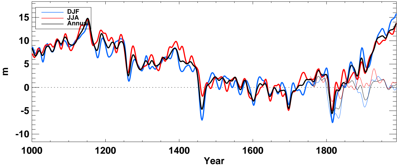
z500_ from echo-g averaged over S-extratropics full
