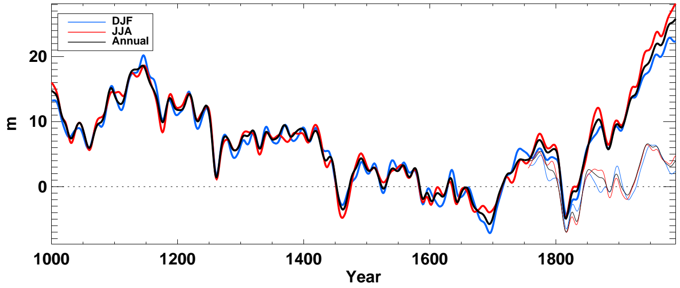
z500_ from echo-g averaged over NH ocean
