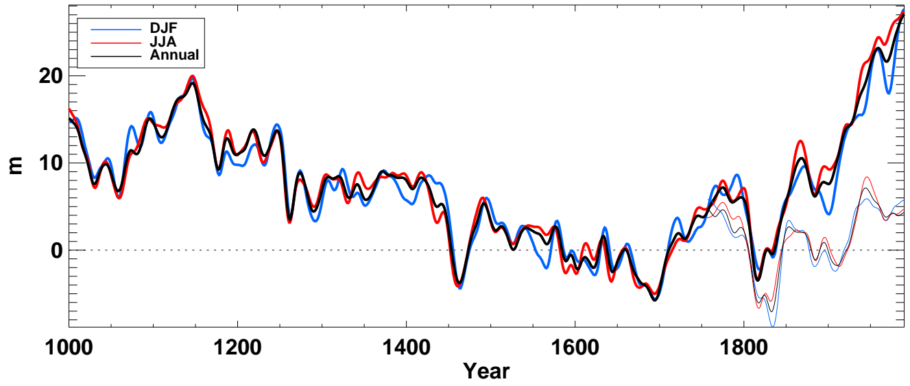
z500_ from echo-g averaged over NH land
