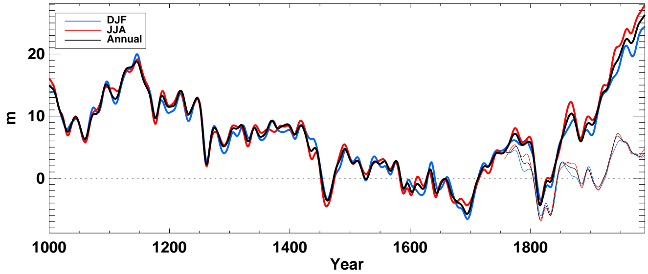
z500_ from echo-g averaged over NH full
