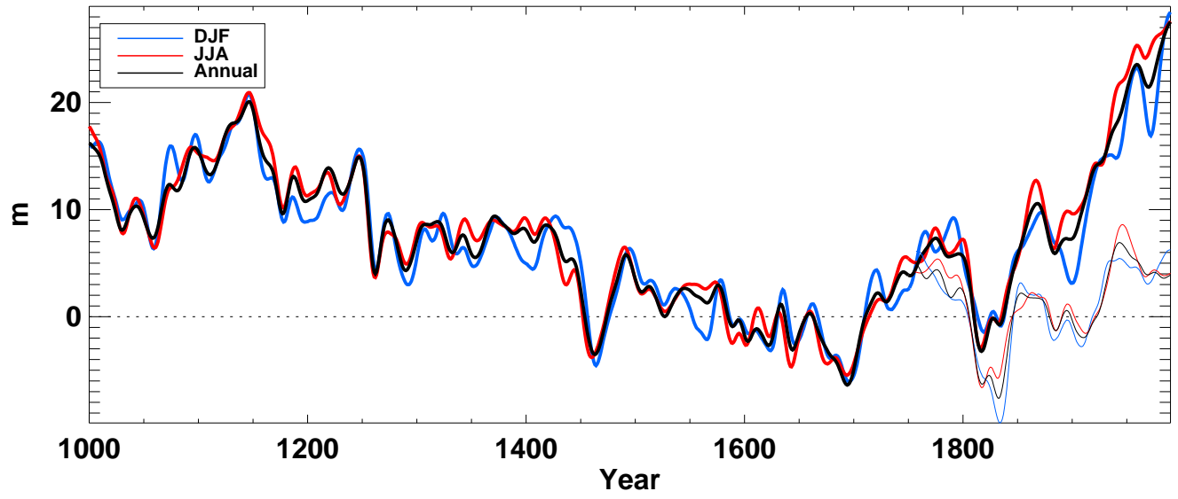
z500_ from echo-g averaged over N-extratropics land
