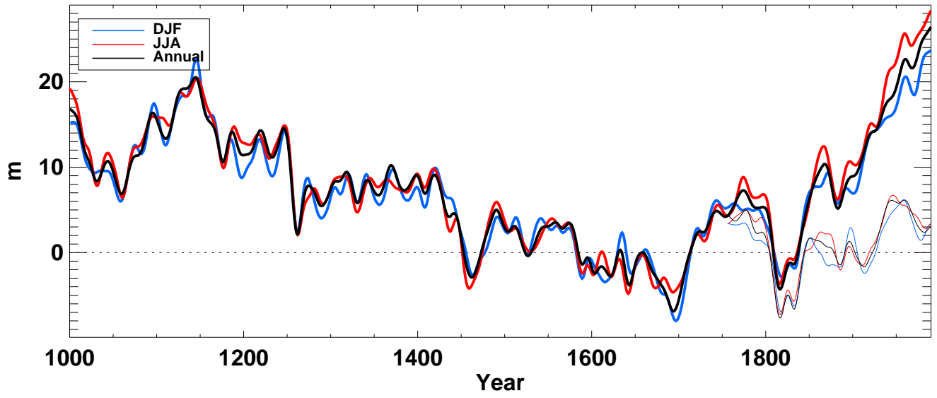
z500_ from echo-g averaged over N-extratropics full
