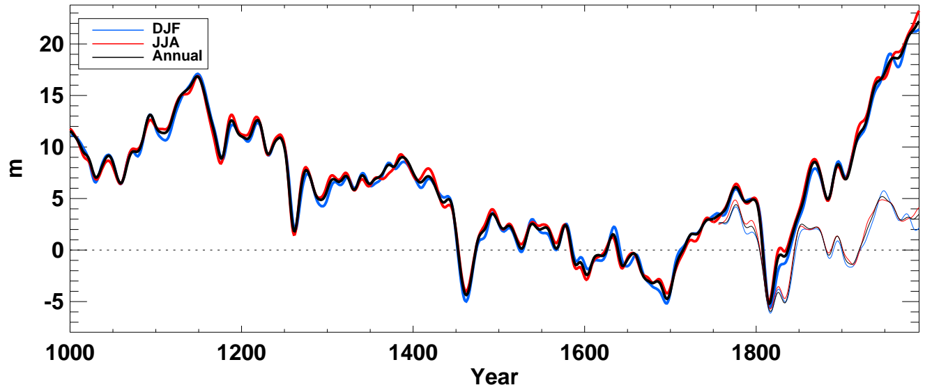
z500_ from echo-g averaged over Global ocean
