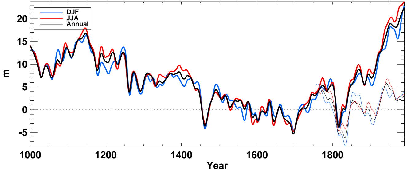
z500_ from echo-g averaged over Global land
