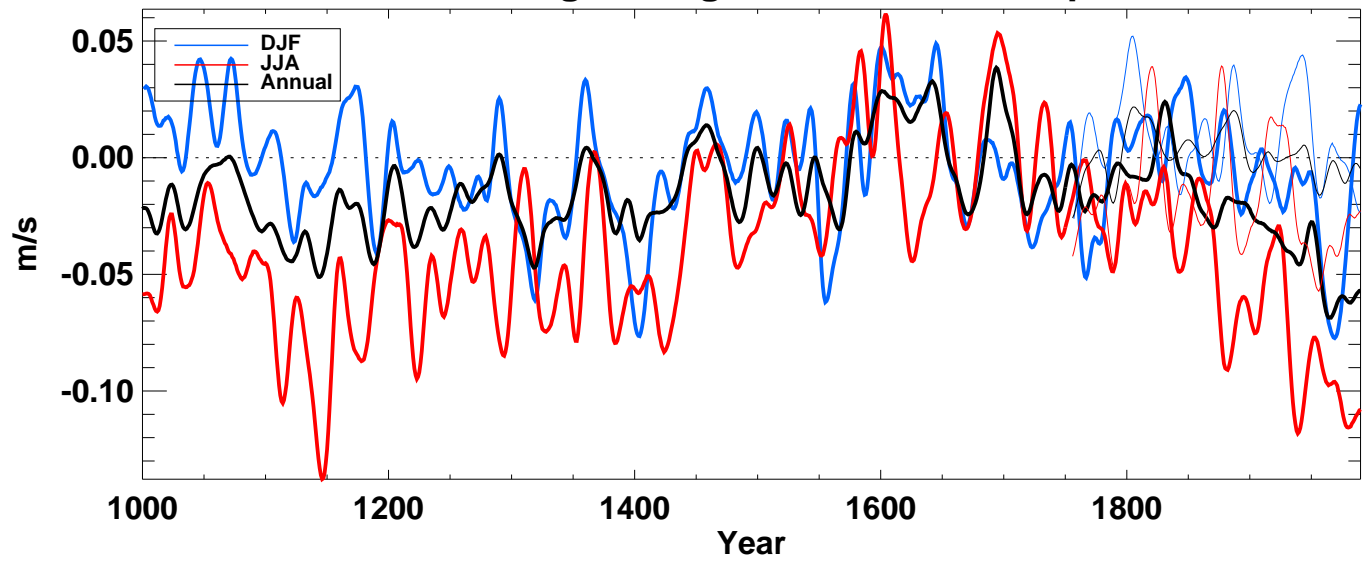
win10 from echo-g averaged over N-extratropics ocean
