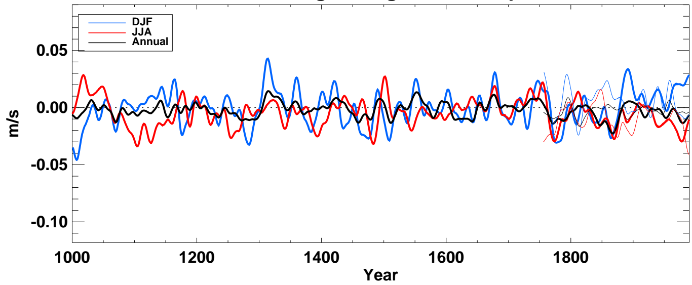
v500_ from echo-g averaged over Tropics ocean
