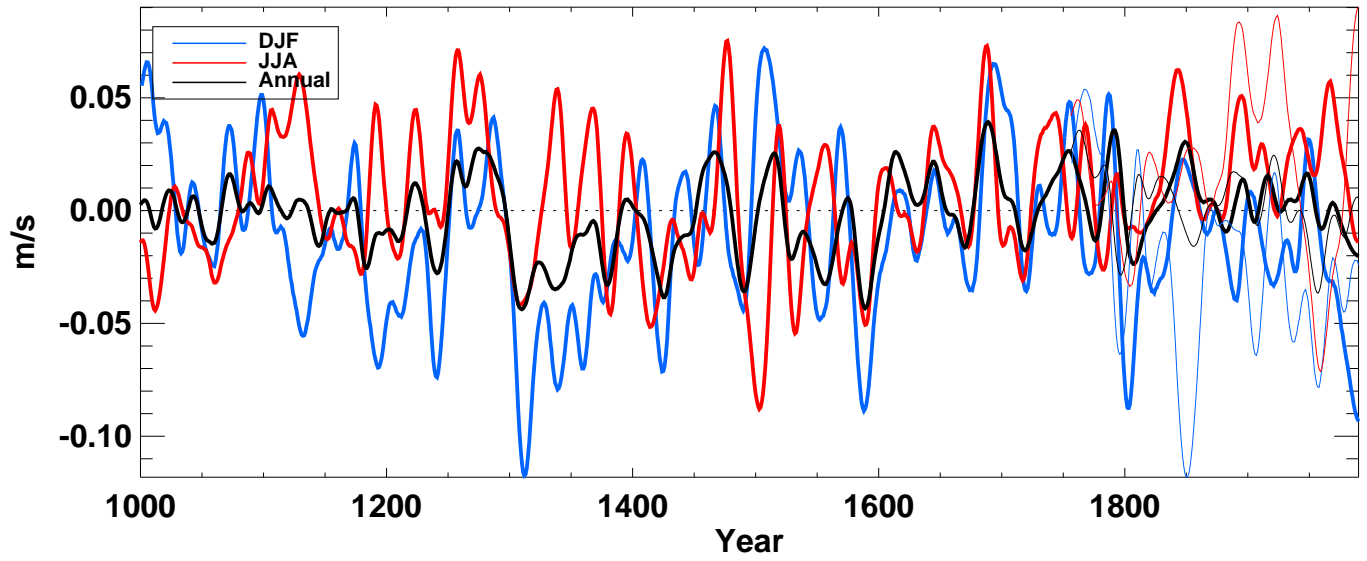
v500_ from echo-g averaged over Tropics land
