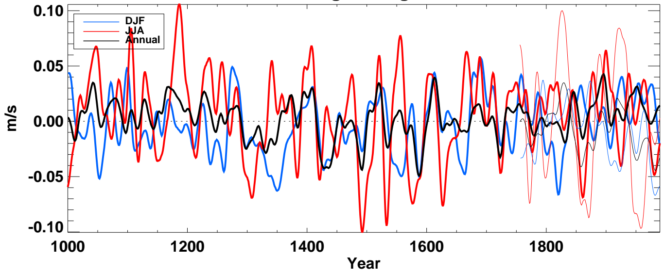
v500_ from echo-g averaged over SH land
