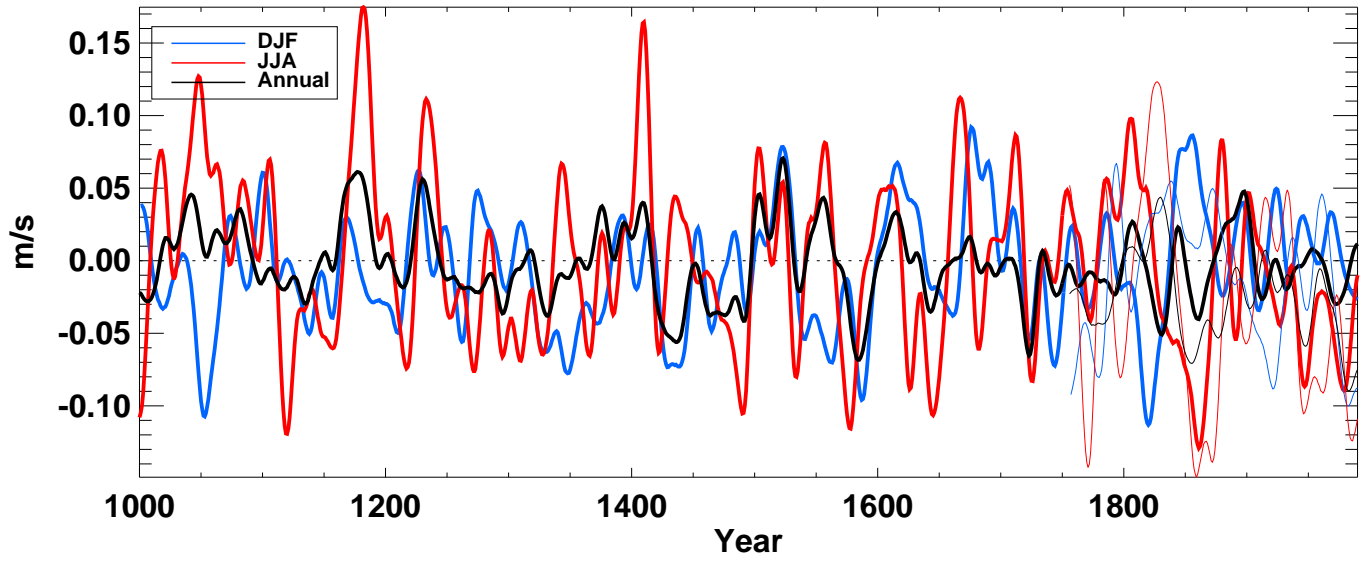
v500_ from echo-g averaged over S-extratropics land
