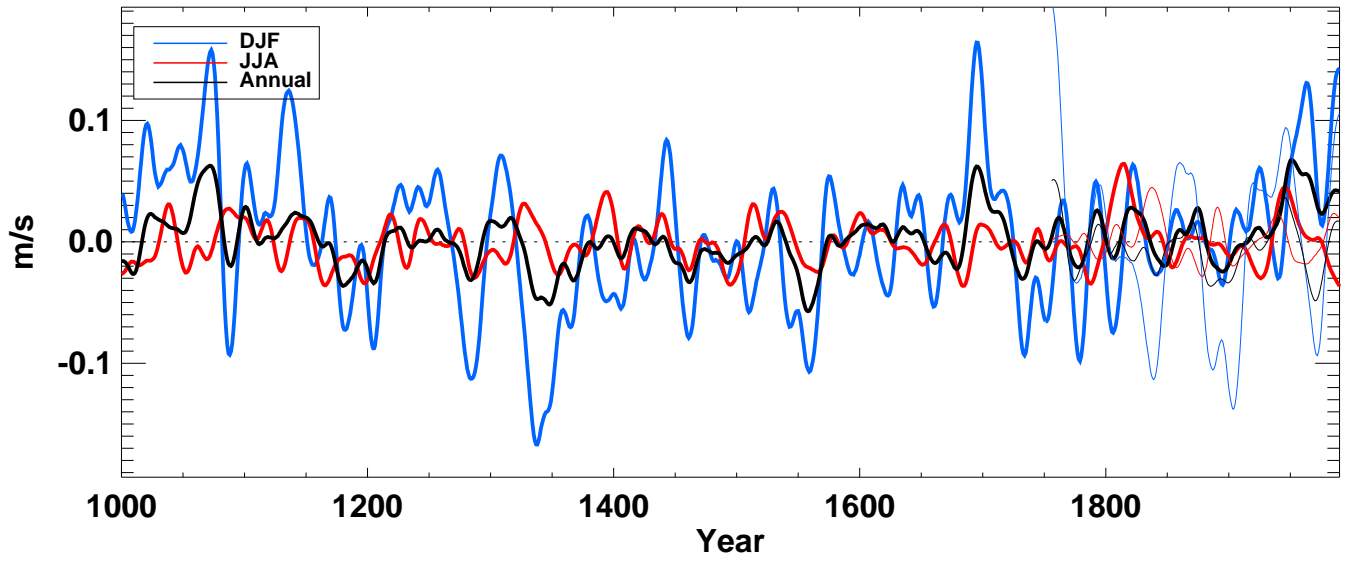
v500_ from echo-g averaged over N-extratropics ocean
