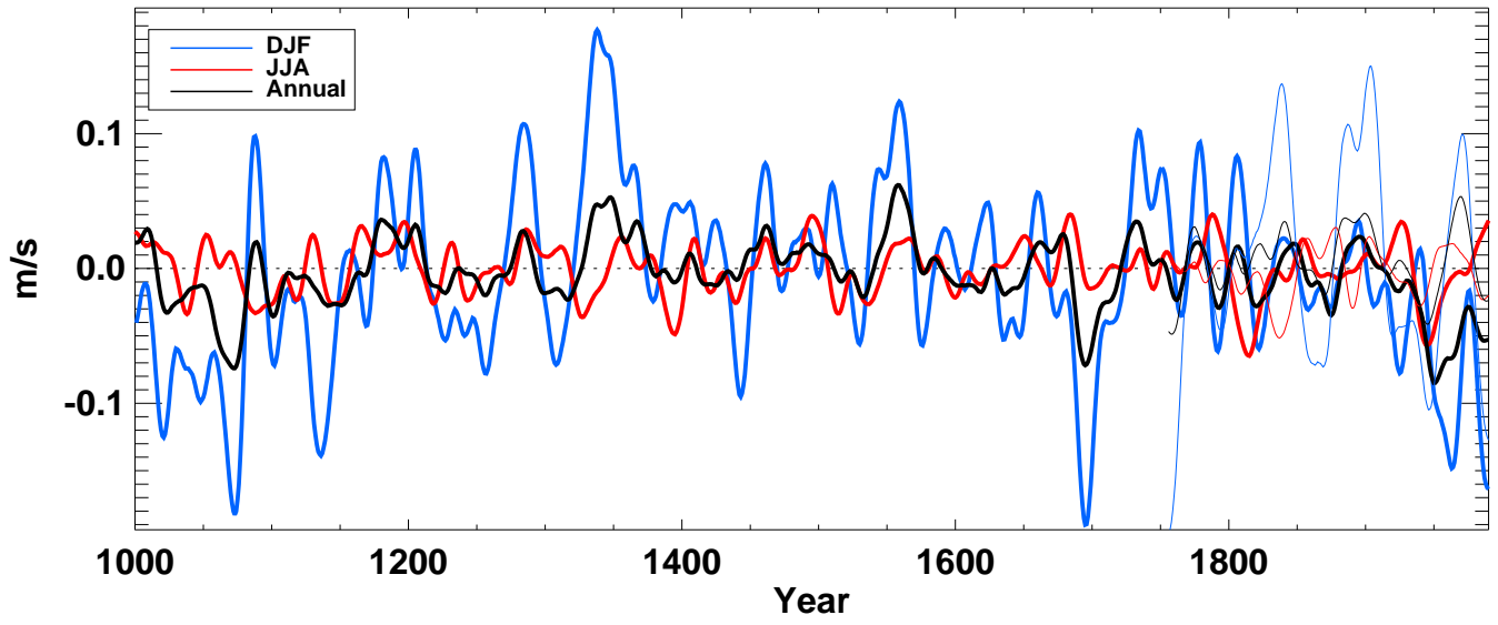
v500_ from echo-g averaged over N-extratropics land
