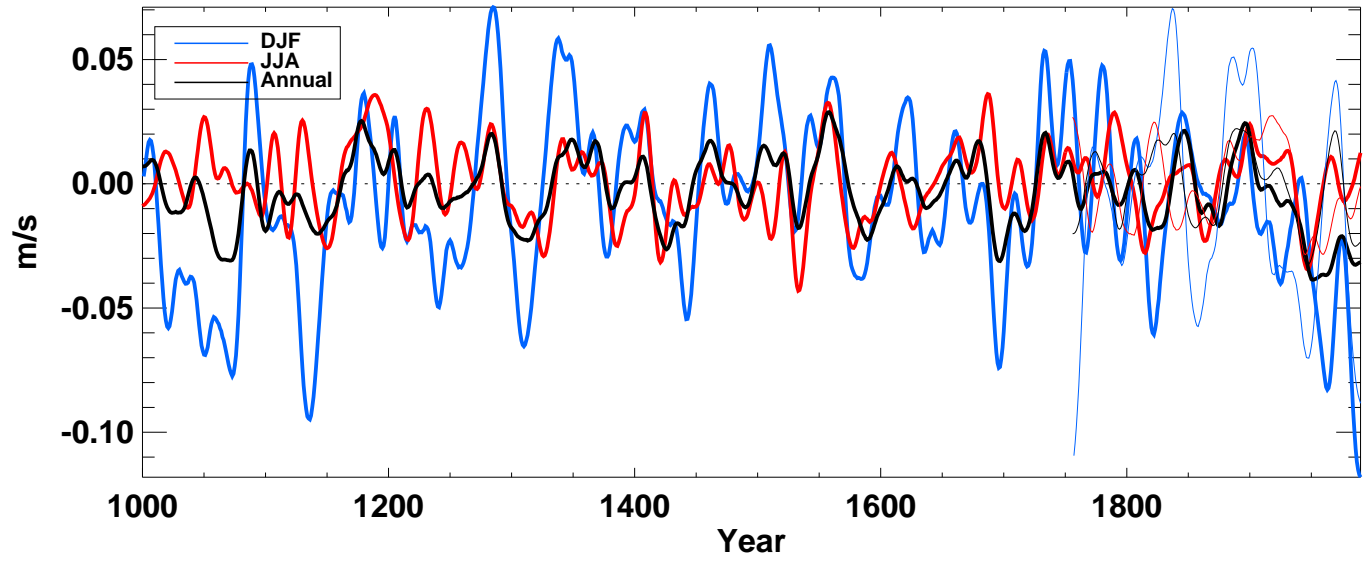
v500_ from echo-g averaged over Global land
