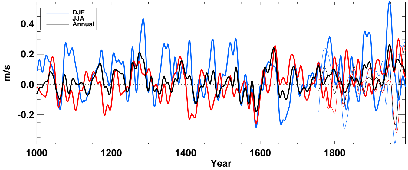
u500_ from echo-g averaged over Tropics ocean
