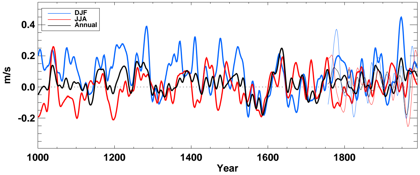
u500_ from echo-g averaged over Tropics land
