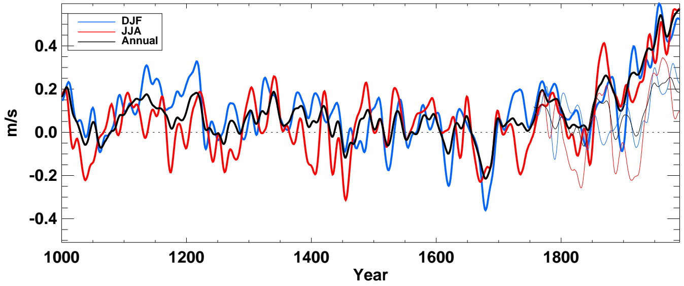
u500_ from echo-g averaged over S-extratropics ocean
