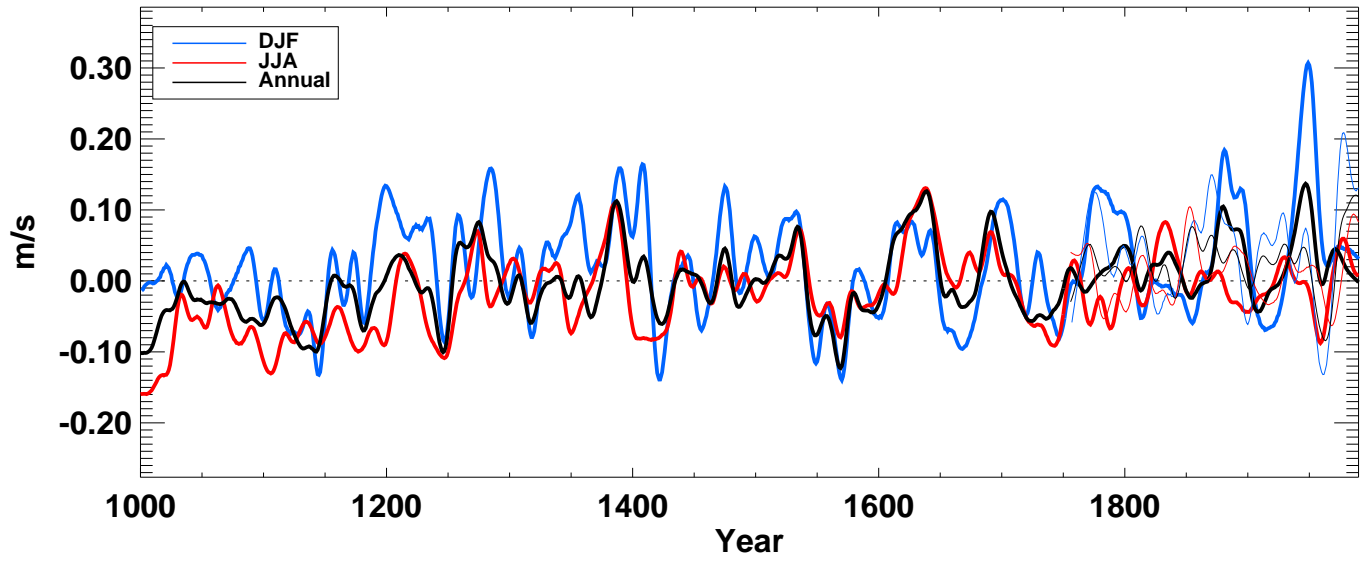
u500_ from echo-g averaged over NH full
