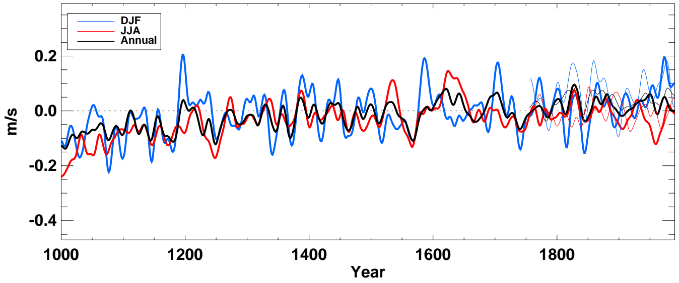
u500_ from echo-g averaged over N-extratropics full
