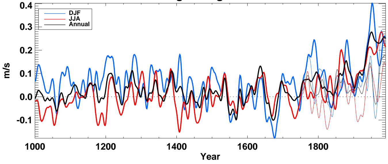
u500_ from echo-g averaged over Global ocean
