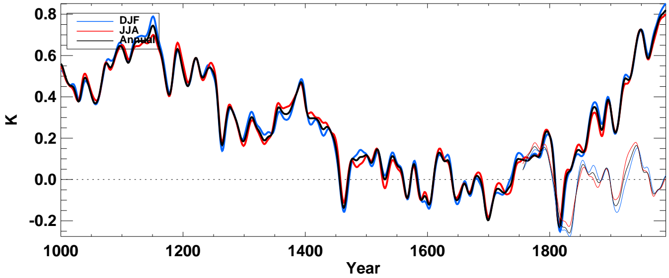
tsoi4 from echo-g averaged over SH land
