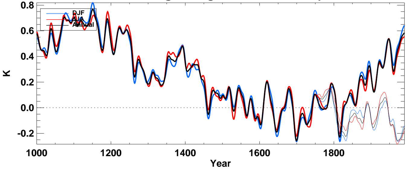
tsoi4 from echo-g averaged over S-extratropics land
