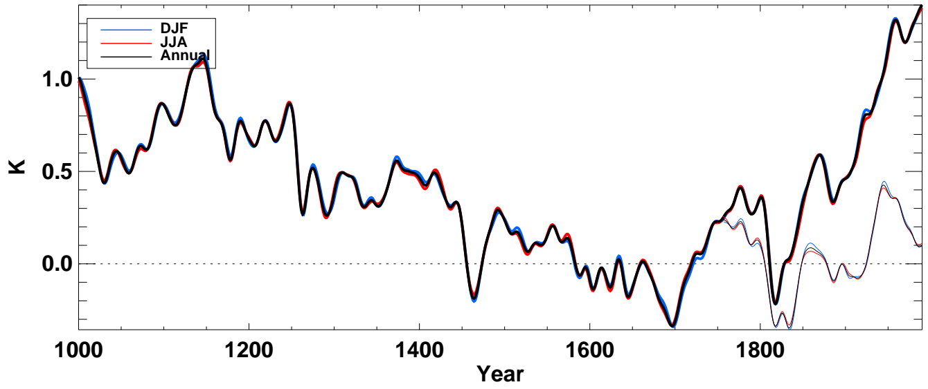
tsoi4 from echo-g averaged over NH land
