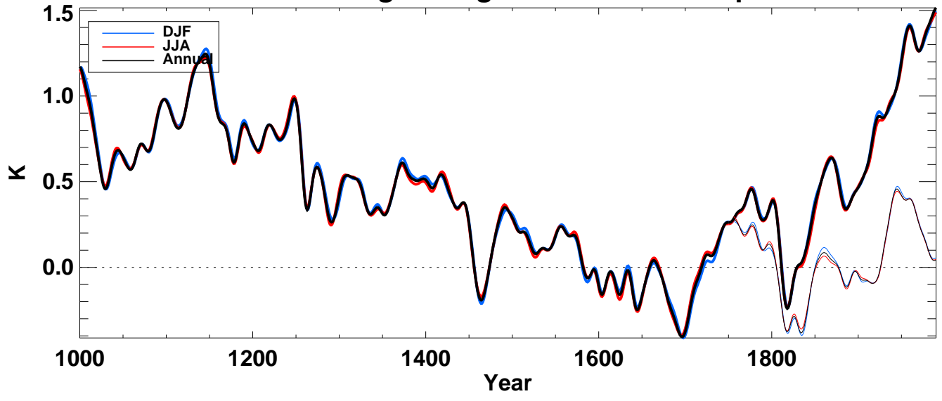
tsoi4 from echo-g averaged over N-extratropics land
