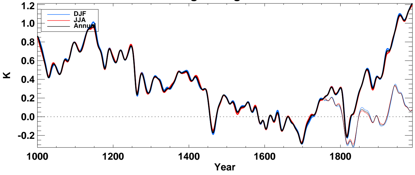
tsoi4 from echo-g averaged over Global land
