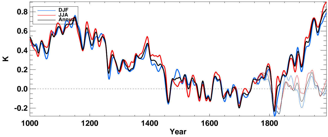
tsoi3 from echo-g averaged over SH land
