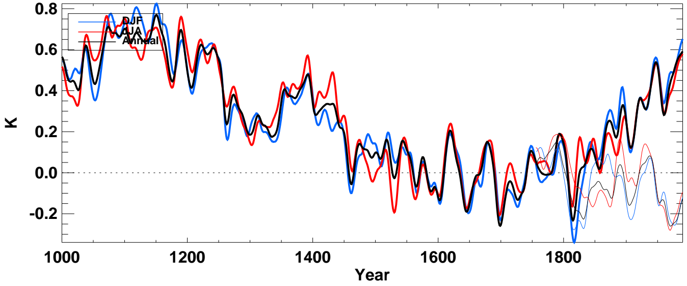
tsoi3 from echo-g averaged over S-extratropics land
