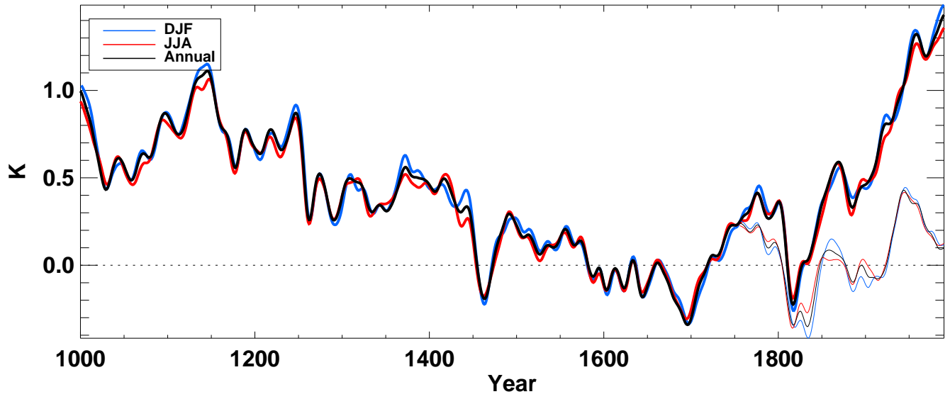
tsoi3 from echo-g averaged over NH land
