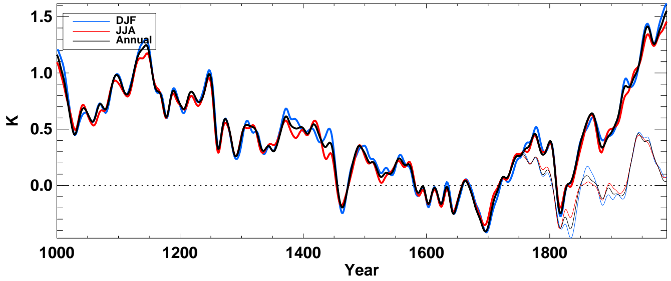
tsoi3 from echo-g averaged over N-extratropics land
