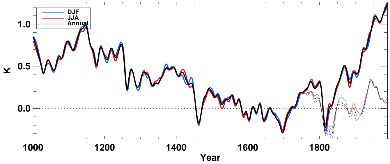
tsoi3 from echo-g averaged over Global land
