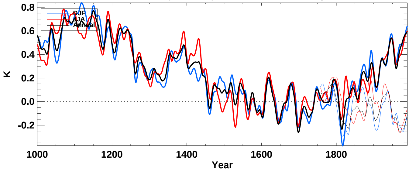
tsoi2 from echo-g averaged over S-extratropics land
