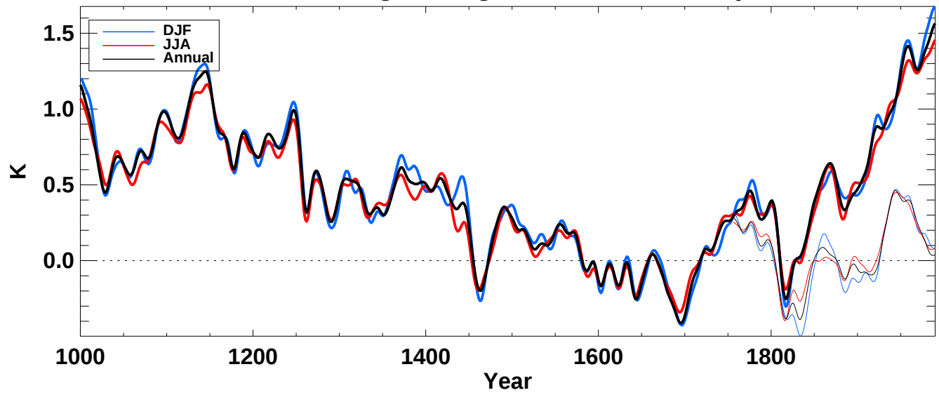
tsoi2 from echo-g averaged over N-extratropics land
