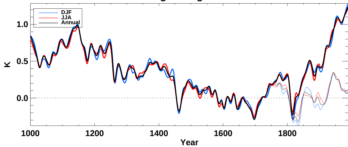
tsoi2 from echo-g averaged over Global land
