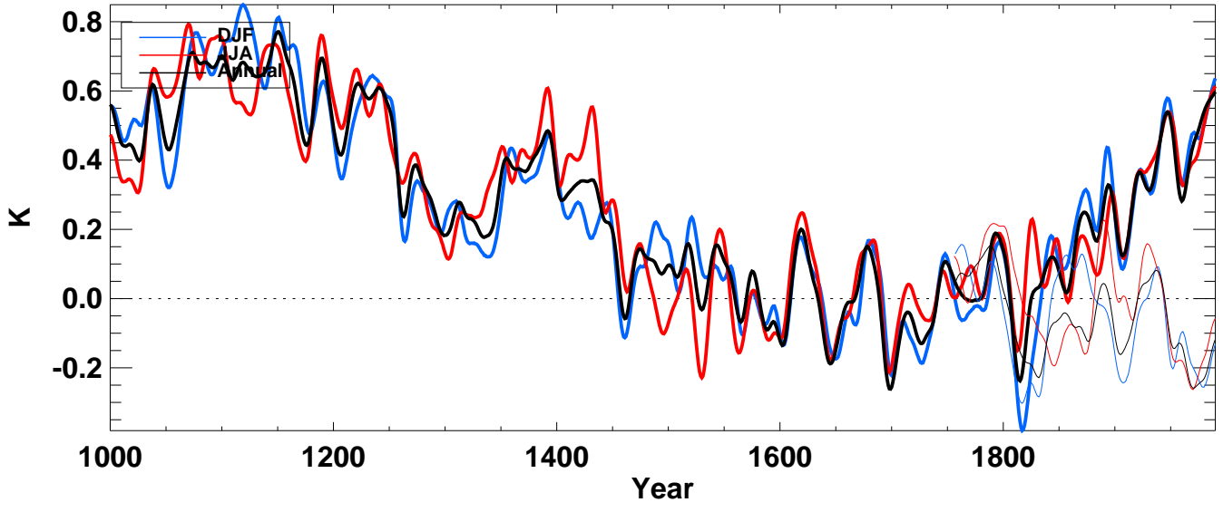
tsoi1 from echo-g averaged over S-extratropics land
