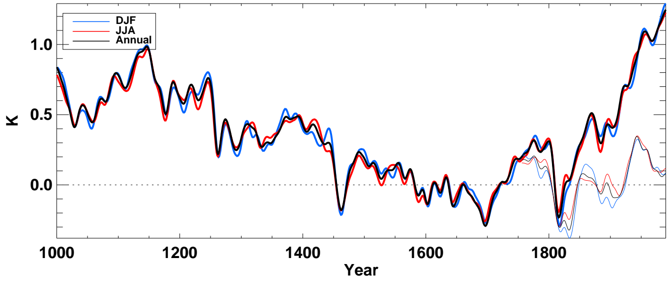
tsoi1 from echo-g averaged over Global land
