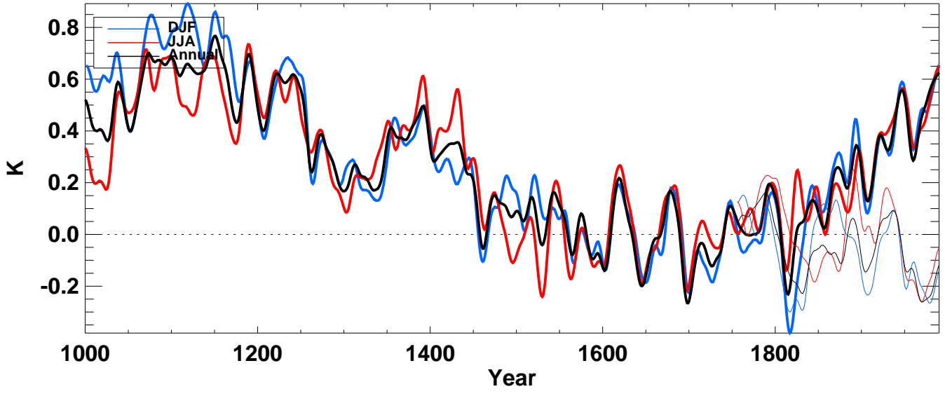
tsnow from echo-g averaged over S-extratropics land
