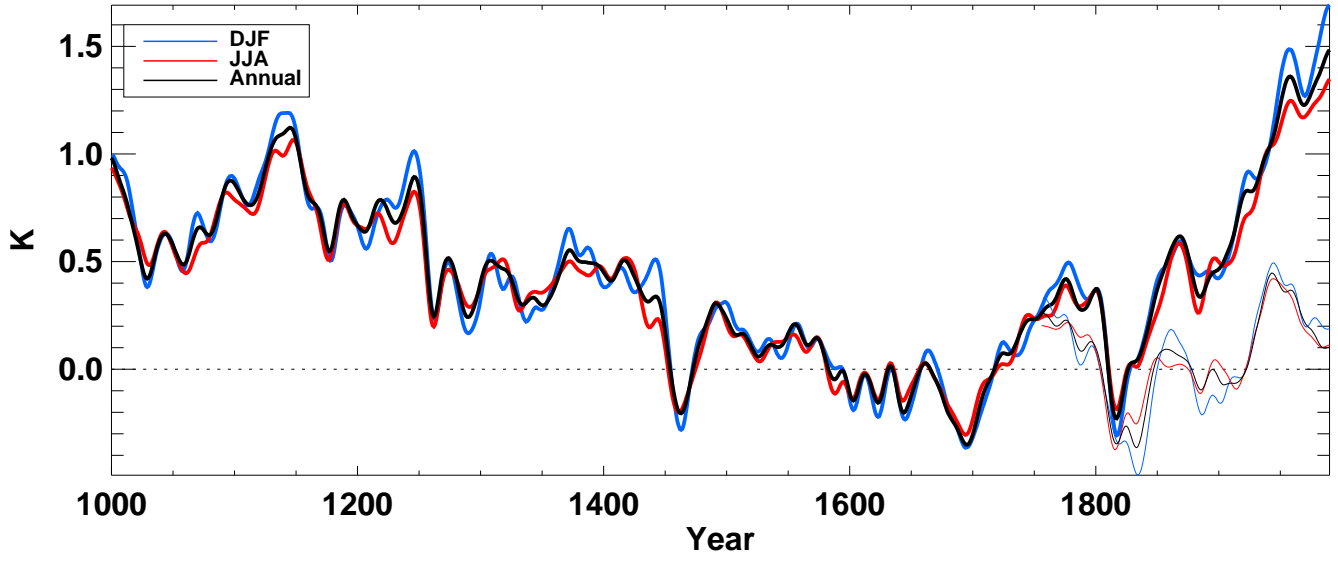
tsnow from echo-g averaged over NH land
