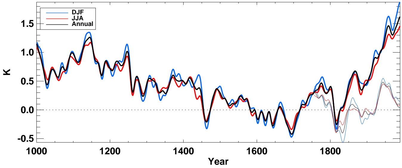
tsnow from echo-g averaged over N-extratropics land
