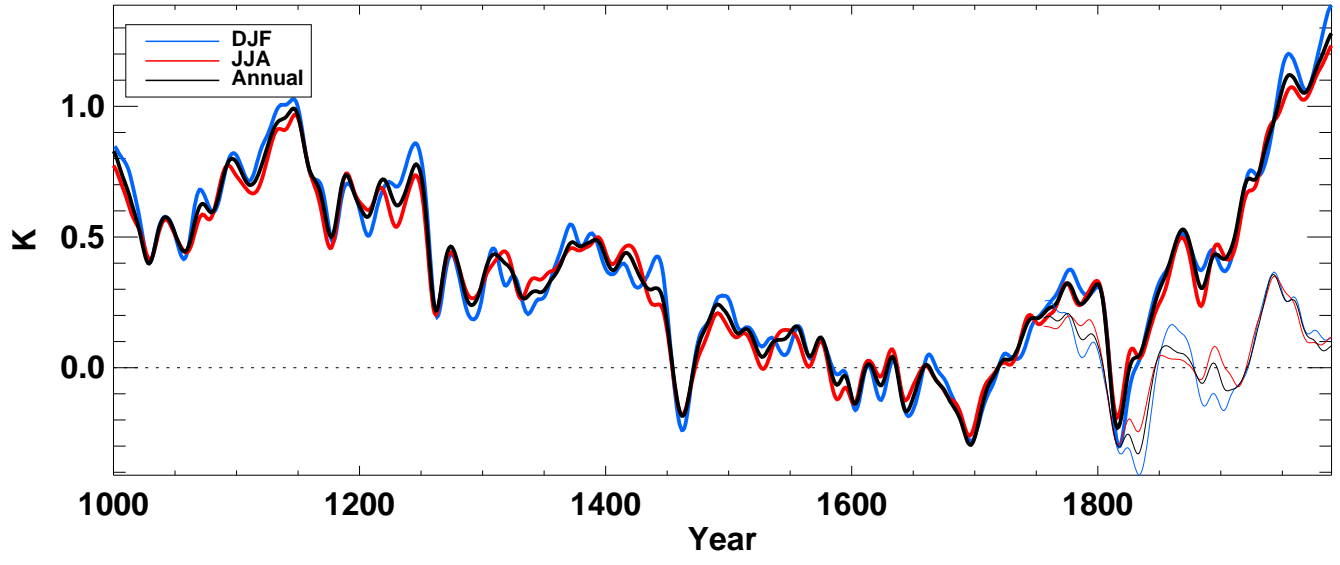
tsnow from echo-g averaged over Global land
