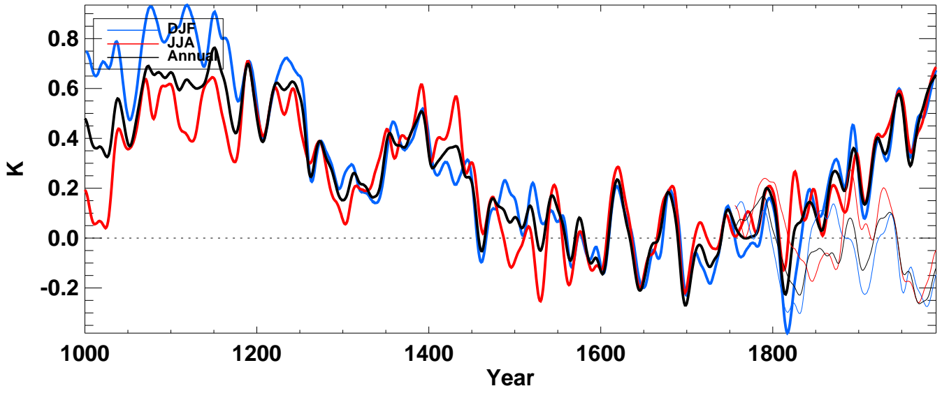
land from echo-g averaged over S-extratropics land
