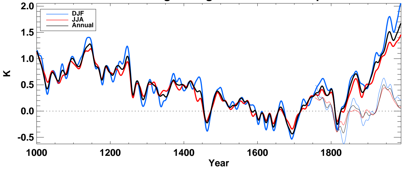
tland from echo-g averaged over N-extratropics land
