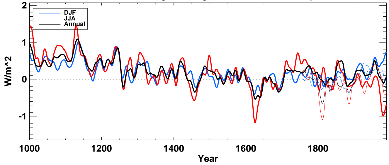
swrad from echo-g averaged over N-extratropics full
