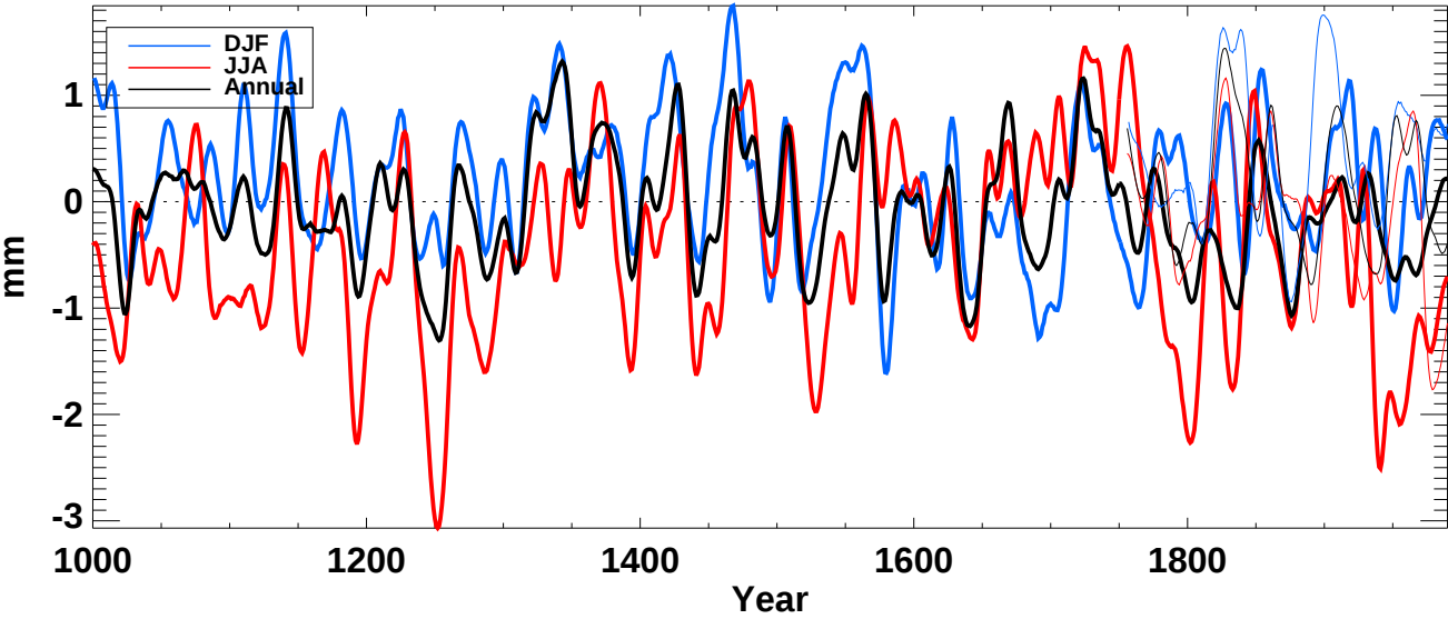
soilm from echo-g averaged over Tropics land
